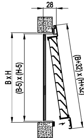
UR2: fixing with magnets
