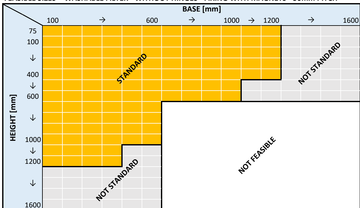
FEASIBLE SIZES - WASHABLE FILTER - WITHOUT HINGES - FIXING WITH MAGNETS - 50mm PITCH
