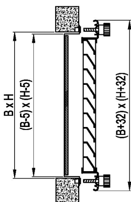
UR24: fixing with knobs
