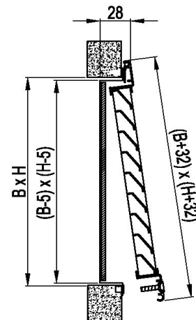
UR3: fixing with screws
