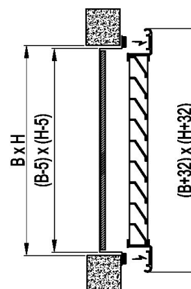
UR22: fixing with magnets
