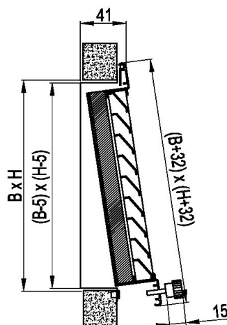
UR14: fixing with knobs
