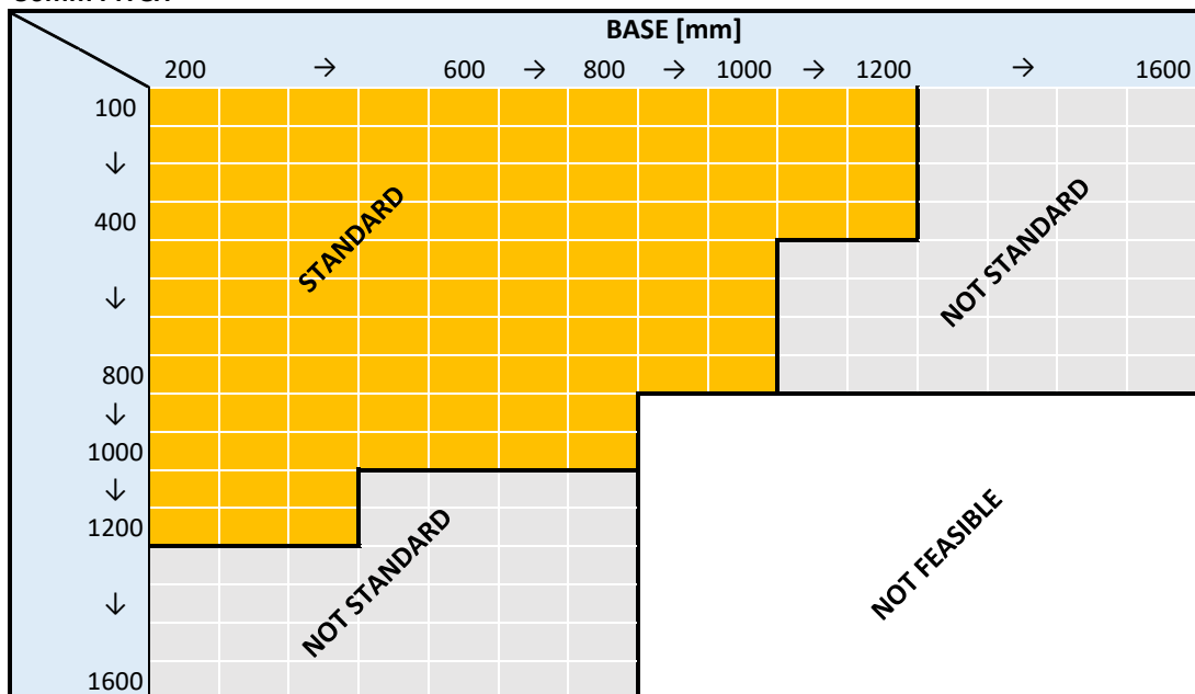
FEASIBLE SIZES - RIGID FILTER - WITHOUT HINGES - FIXING WITH CLIPS 50mm PITCH
