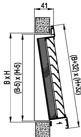
UR12: fixing with magnets
