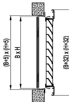
UR21: fixing with clips
