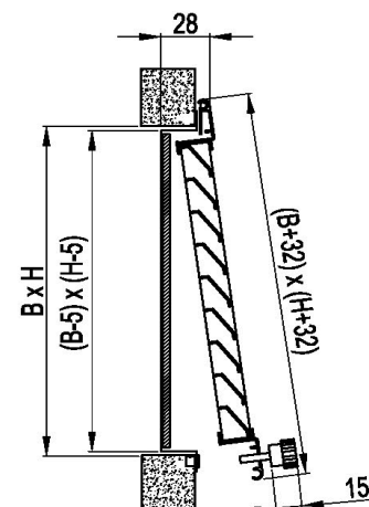
UR3: fixing with screws
