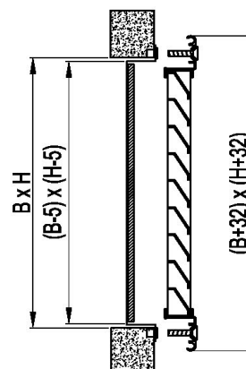
UR23: fixing with screws
