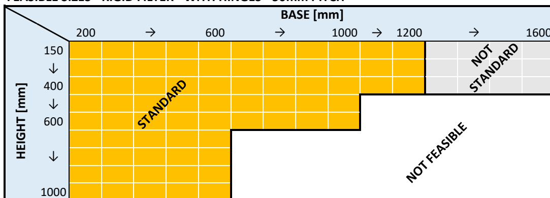
FEASIBLE SIZES - RIGID FILTER - WITH HINGES - 50mm PITCH
