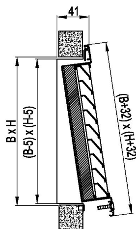
UR13: fixing with screws
