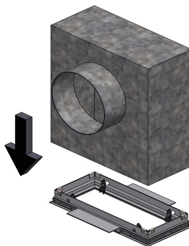
2 - Insert the concealed frame inside the plenum
