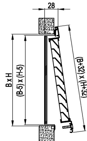
UR3: fixing with screws
