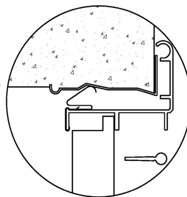
Mounting with double deflection grille
