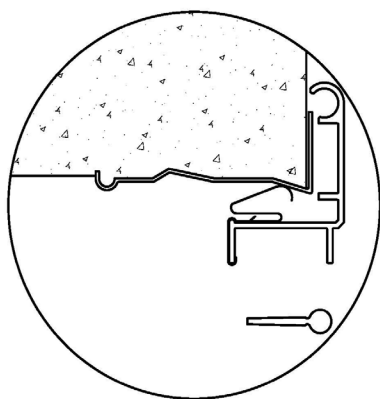
Mounting with single deflection grille
