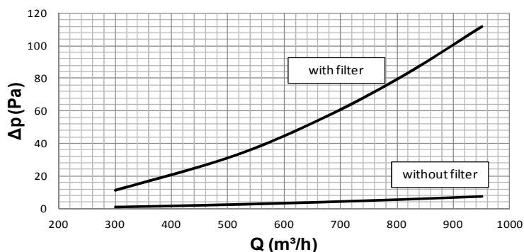
KNF 2 600x600 - pressure drop - return
