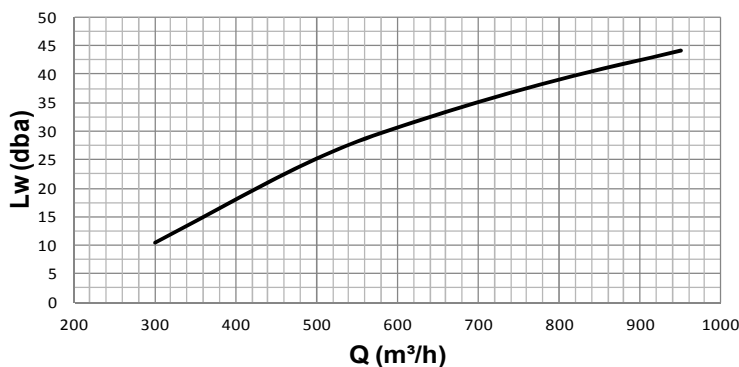
KNF 2 600x600 - sound power
