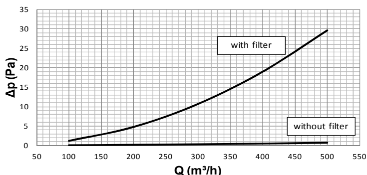
KNF 1 675x675 - pressure drop - return
