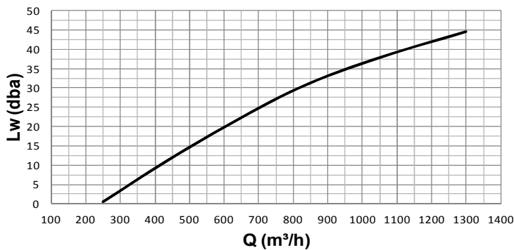
KNF 3 675x675 - sound power
