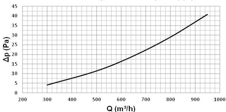
KNF 2 600x600 - pressure drop - supply
