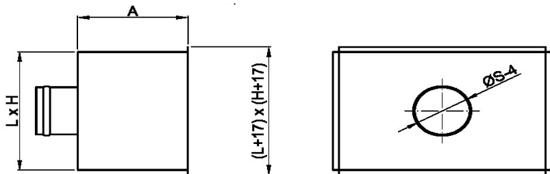
GRILLE WITH FILTERHOLDER FRAME
