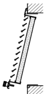
with rigid filter fixing hinge and knob Installation on wall or ceiling
