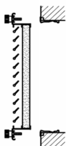
with rigid filter fixing both sides with knobs Installation on wall or ceiling
