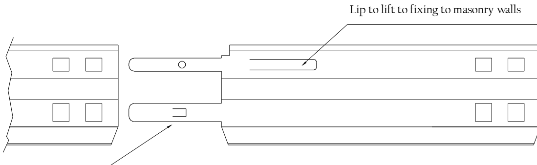
blades to bend at 90° and insert in the attaching part to assemble the counterframe
